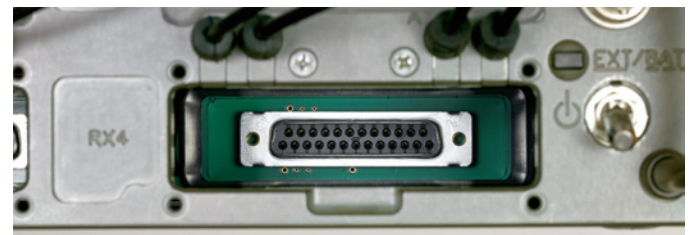
Receivers interface with the Octopack board via a 25-pin connector and the Unislot adapter.
