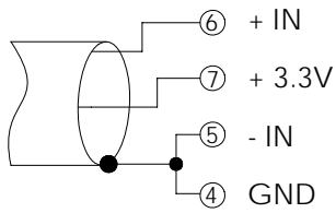
Electret 3 wires
