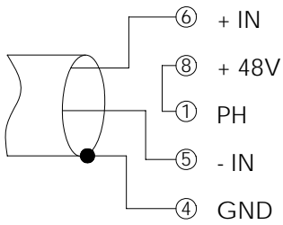
Microphone 48V Phantom
