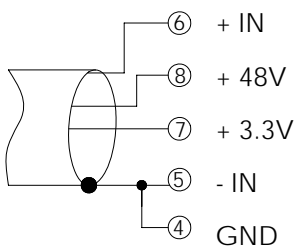
Microphone Schoeps active cable
